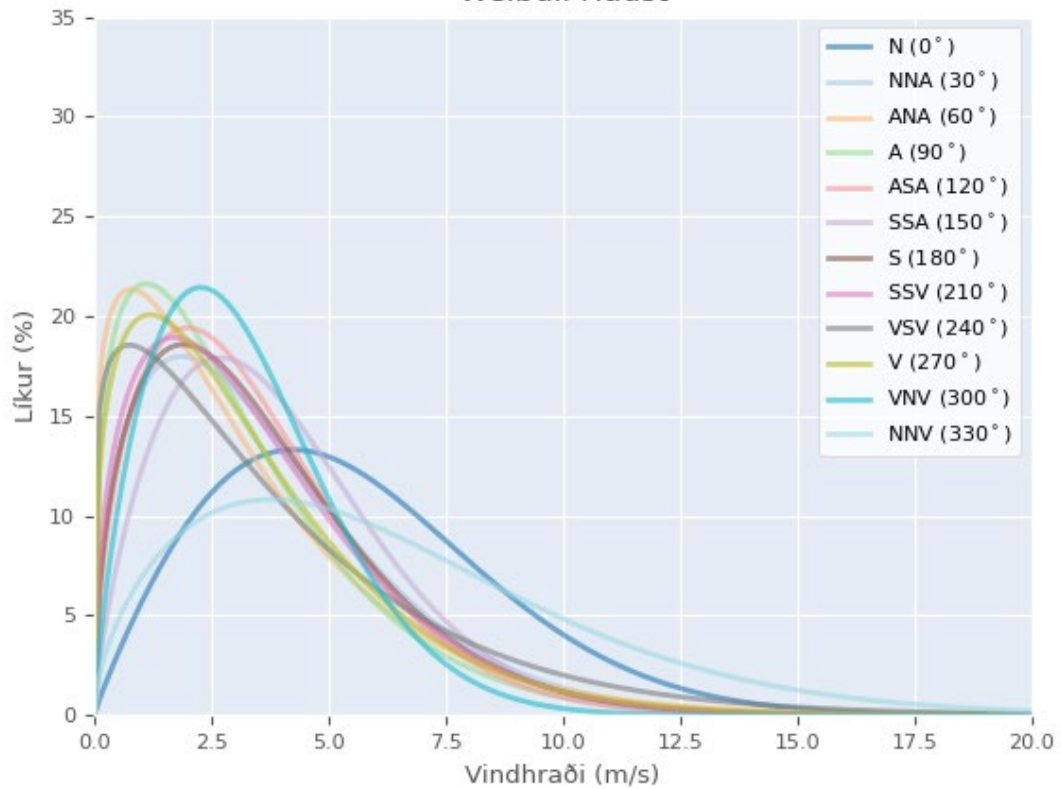
Weibull Haust
